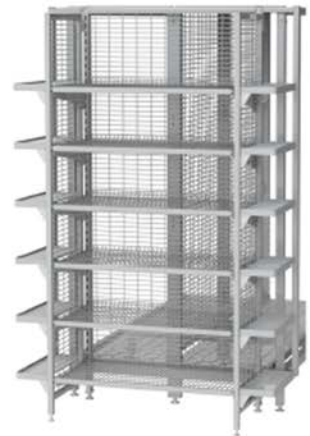
POSITION 4 Folded out with centre + side shelves Freestanding
